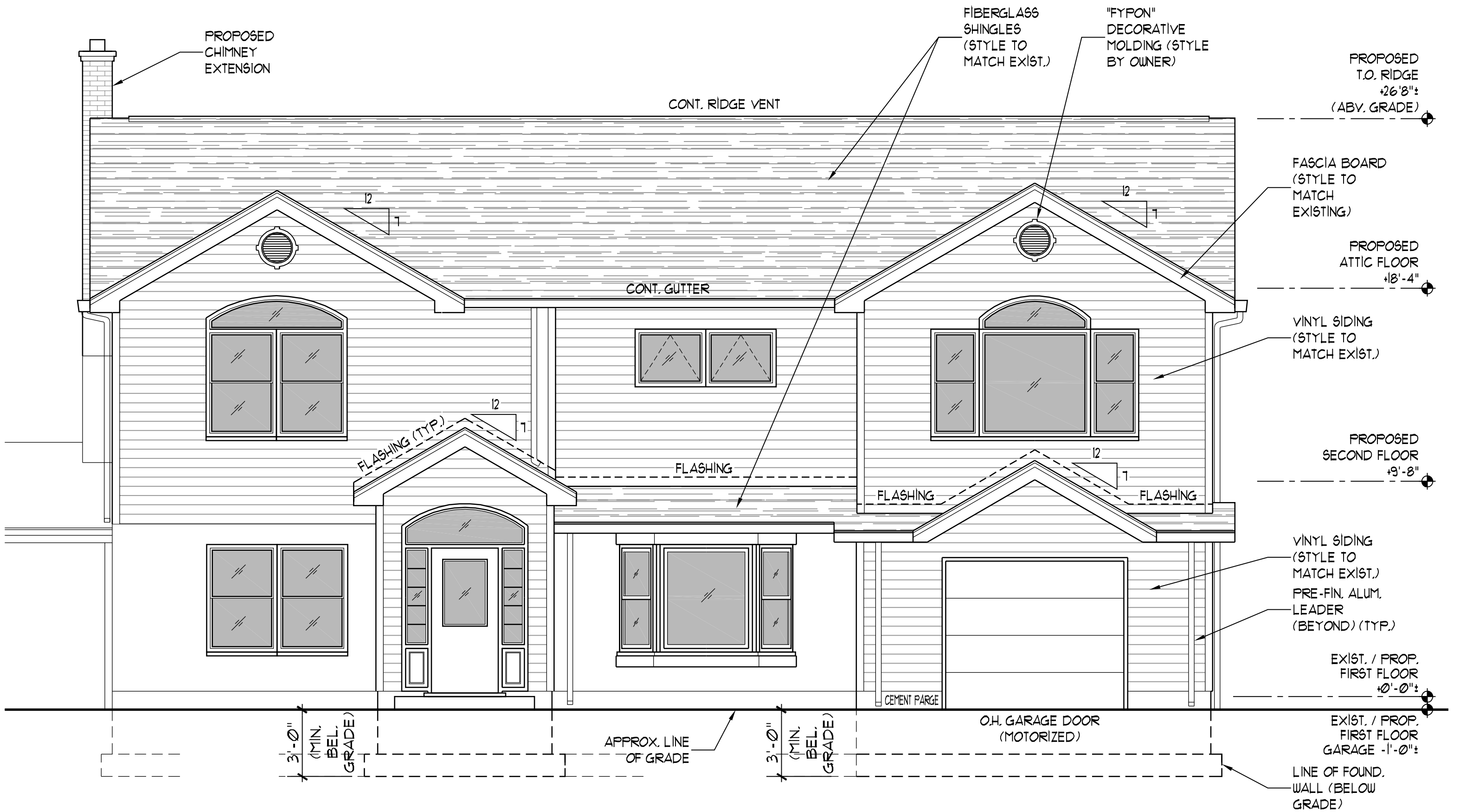
1 PROPOSED FRONT ELEVATION 1/4" = 1'-0"
