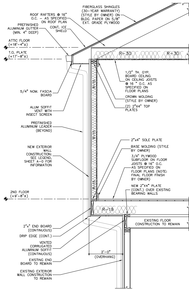
3 TYP. WALL SECTION 3/4" = 1'-0"
