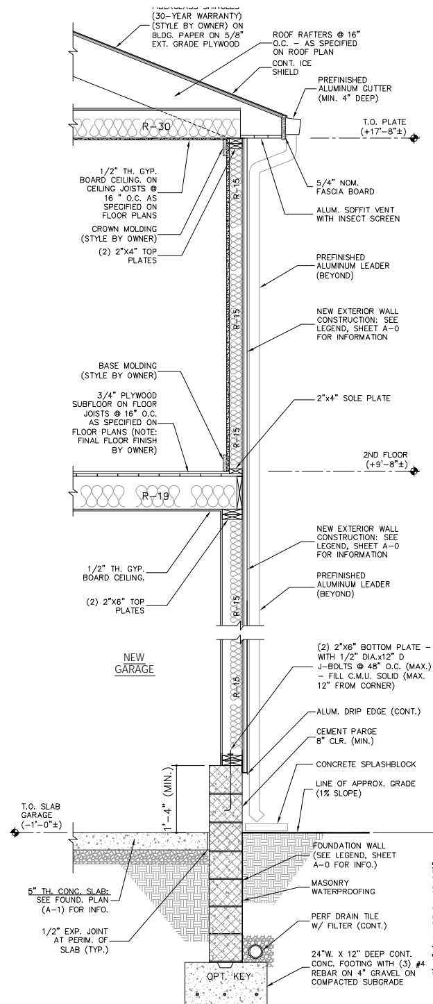
2 TYP. WALL SECTION 3/4" = 1'-0"
